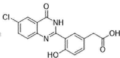
2-(3-(6-chloro-4-oxo-3,4-dihydroquinazolin-2-yl)-4-
