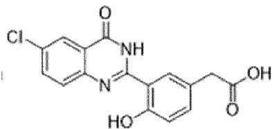
2-(3-(6-chloro-4-oxo-3,4-dihydroquinazolin-2-yl)-4-hydroxyphenyl)acetic acid (11) .
