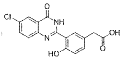
2-(3-(6-chloro-4-oxo-3,4-dihydroquinazolin-2-yl)-4-
